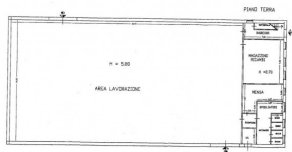
PIANO TERRA SCALA 1: 200
