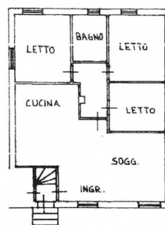
PIANO TERRA h= 293
